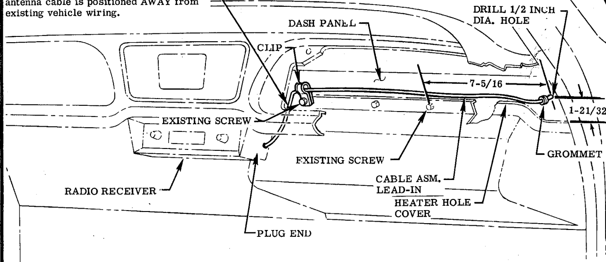
FIG. 4 CABLE ASSY. LEAD-IN
